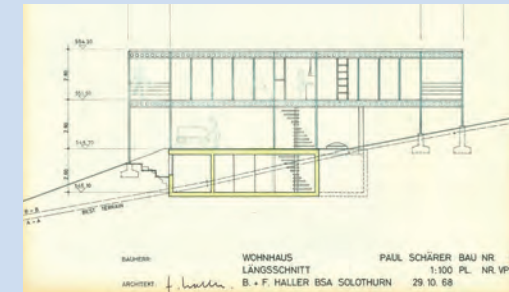
Plan original Fritz Haller, 1968
